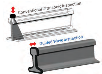
Unlike conventional ultrasonic inspection, guided waves provide 100% volumetric inspection and can inspect tens of metres in a single test.
